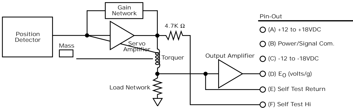
Block Diagram for the LSO Inclinometer
