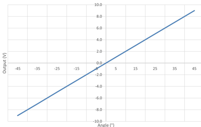
LCH-A-S-45-10 (V1 - V2 Differential Output)
