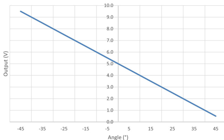
LCH-A-S-45-10 (V2 Output)
