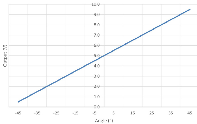
LCH-A-S-45-10 (V1 Output)
